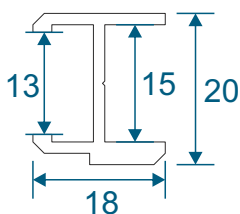
SG58 - 4 Pane Meeting Stile
